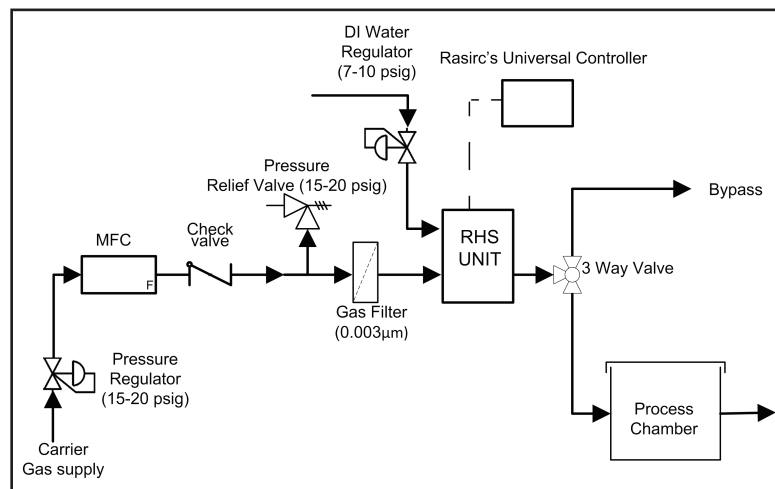
Figure 2: RHS Recommended Installation P&ID
