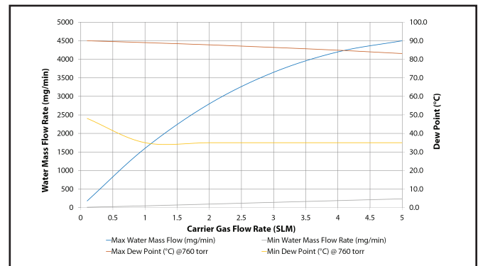
Figure 4: RHS Low Flow Unit Control Range
