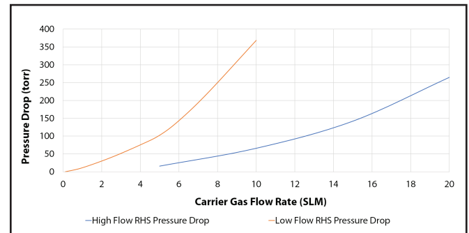
Figure 5: Water Vapor Pressure Drop vs Flow
