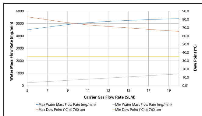
Figure 3: RHS High Flow Unit Control Range
